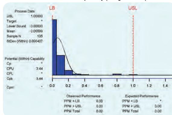
AcuGrav™ Process Capability (Weight Result)
