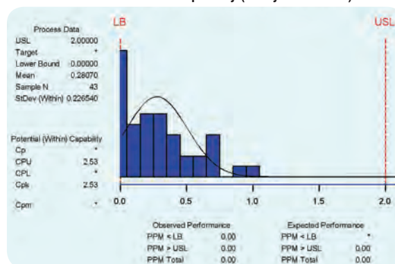
AcuGrav™ Process Capability (Analytical Result)
