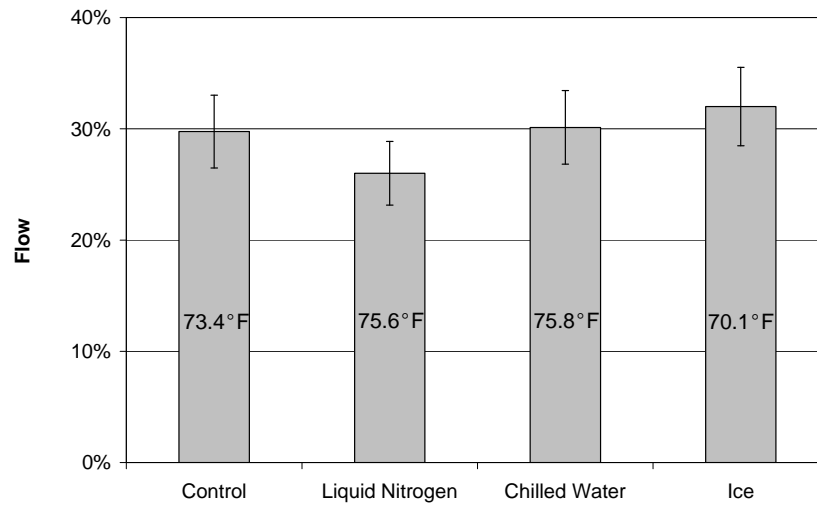
Figure 3.1 Flow of cement mortar containing no admixture
