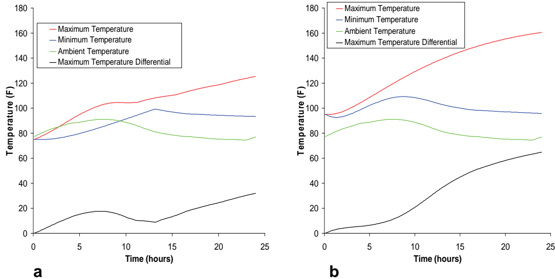
Figure 2.2 Temperature profiles over time of the columns shown in Figure 2.1 (a) 75°F (23.9°C) placement temperature, (b) 95°F (35°C) placement temperature (courtesy of Kyle Riding)
