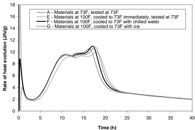
Figure 5.5 Heat evolution curves for isothermal calorimetry Mixture 4, A and E-G (C ash)
