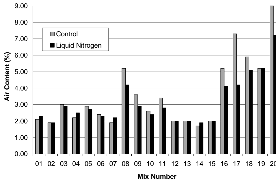
Figure 7.1 Fresh air contents for laboratory-mixed concrete
