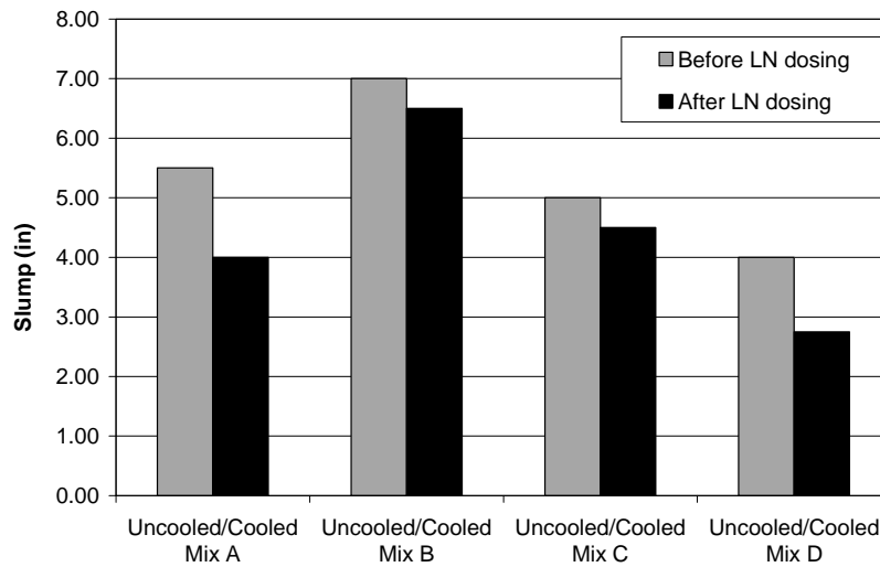
Figure 3.7 Slump results for field-mixed concrete
