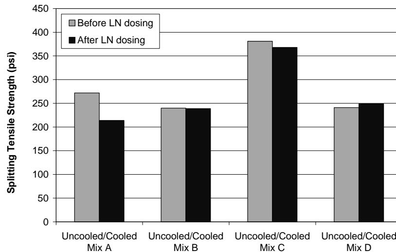
Figure 4.6 Splitting tensile strength for field-mixed concrete
