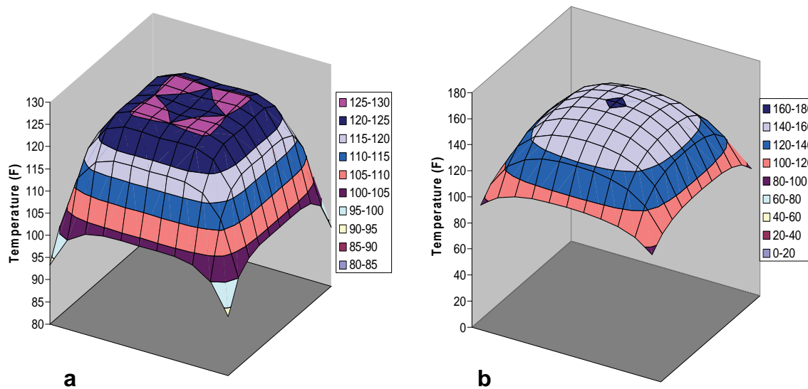
Figure 2.1 Examples of the temperature distribution in a horizontal cross section of a 7ft. by 7ft. column at 24 hours (a) 75°F (23.9°C) placement temperature, (b) 95°F (35°C) placement temperature (courtesy of Kyle Riding)
