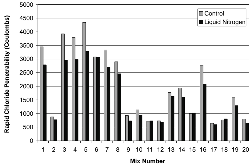
Figure 4.8 Rapid chloride penetrability data for control and liquid nitrogen mixtures
