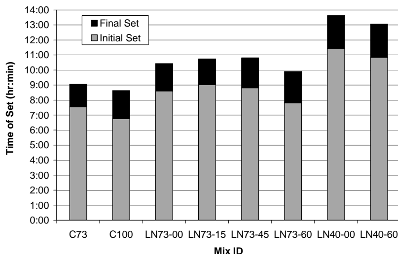
Figure 6.6 Initial and final set times for concrete mixtures delayed dosing mixtures
