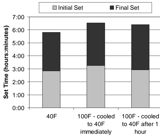
Figure 6.3 Setting time of cement pastes with initial temperatures of 40°F and 100°F, cooled to 40°F immediately or after a 1 hour delay
