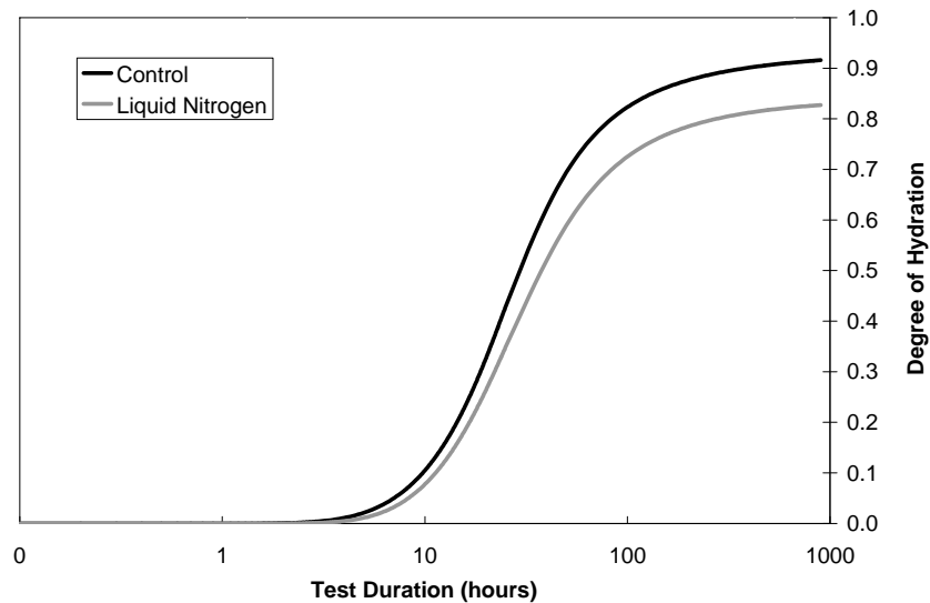
Figure 5.3 Degree of hydration curves for Mixture 19 (C ash + polycarboxylate superplasticizer + air entrainer)
