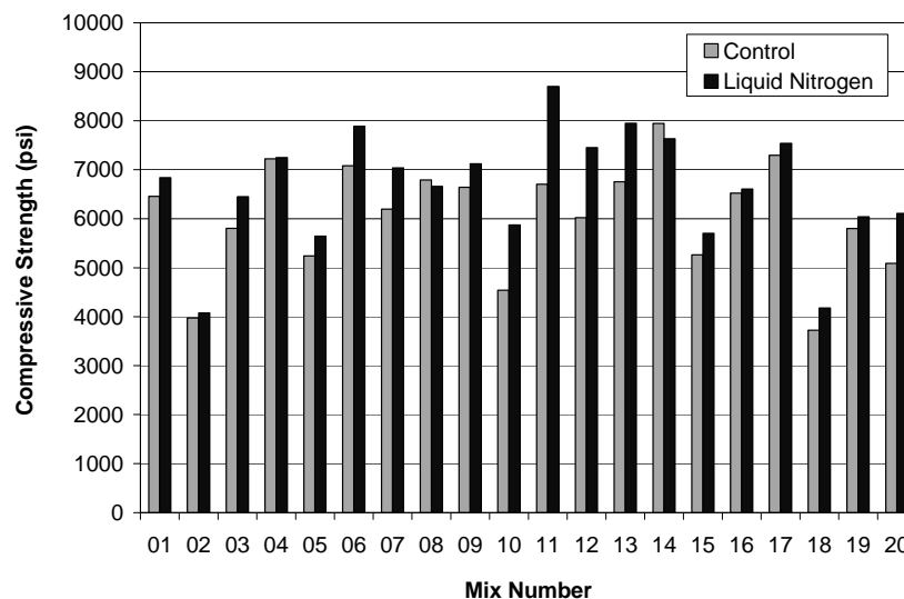
Figure 4.2 28-day compressive strengths for laboratory-mixed concrete
