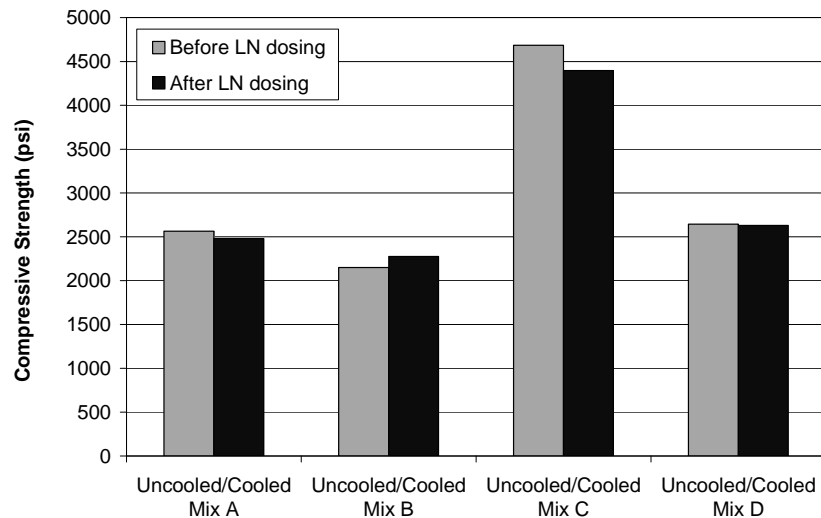
Figure 4.4 28-day compressive strengths for field-mixed concrete
