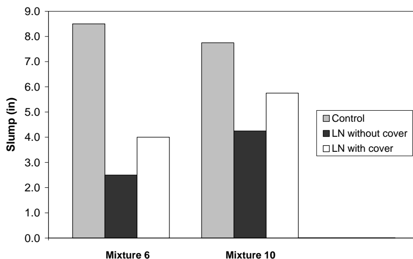
Figure 3.6 Slump comparison of room temperature, covered, and uncovered concrete
