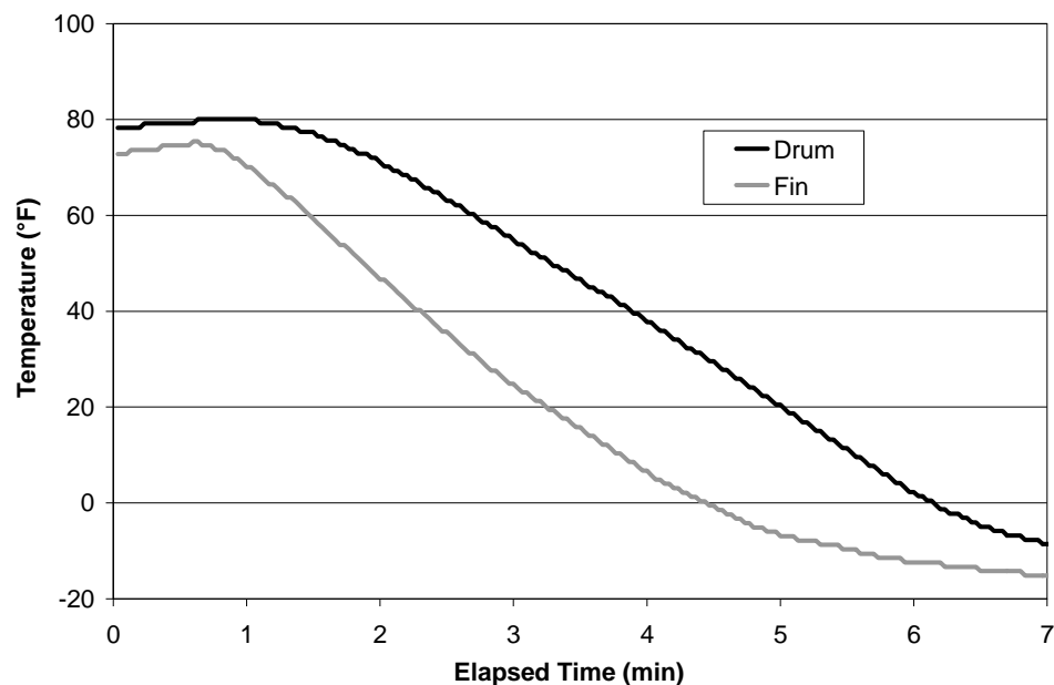
Figure 8.5 Temperature of mixing drum and fin during LN dosing (Truck 5)
