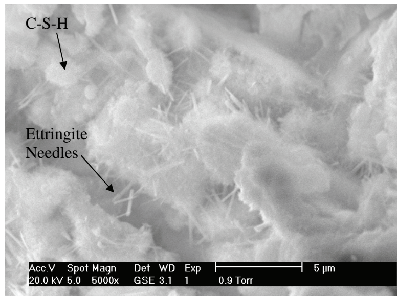
Figure 5.12 ESEM image of fractured cement paste surface from mixture C100 after 24 hours of hydration
