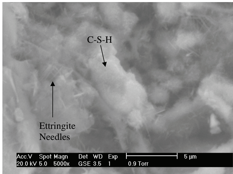
Figure 5.15 ESEM image of fractured cement paste surface from mixture LN50-00 after 24 hours of hydration
