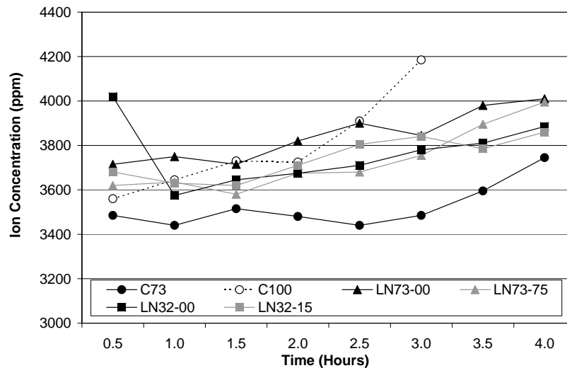
Figure 5.11 Potassium concentrations for six different cement paste mixtures
