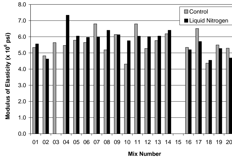
Figure 4.7 Modulus of elasticity comparison for control and liquid nitrogen mixes
