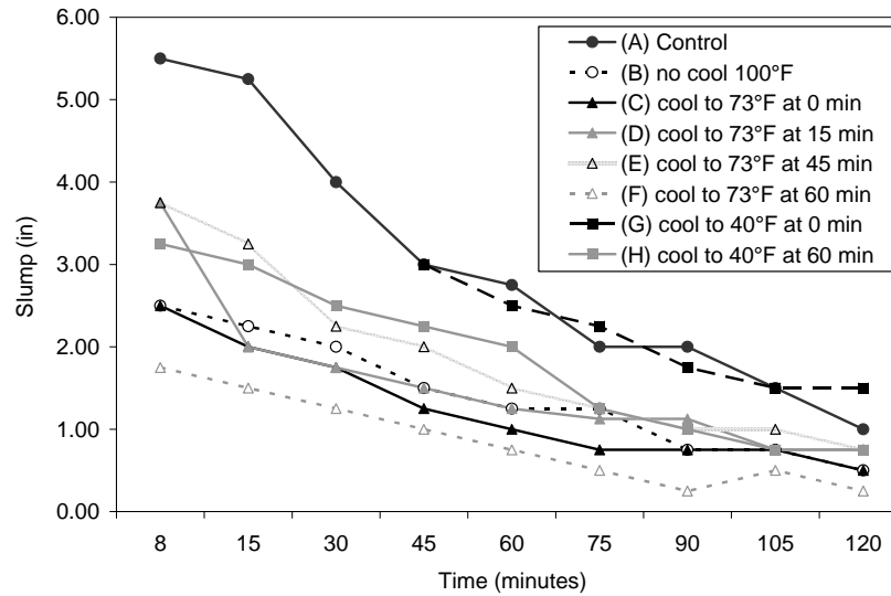
Figure 3.8 Slump retention for concrete mixtures cooled with liquid nitrogen to varying temperatures and at varying time
