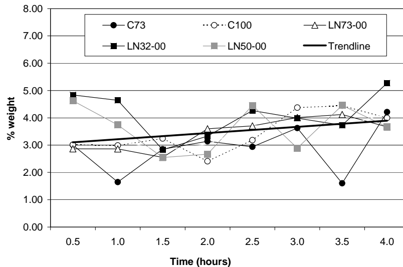
Figure 5.6 Ettringite analyses by x-ray diffraction for five mixtures
