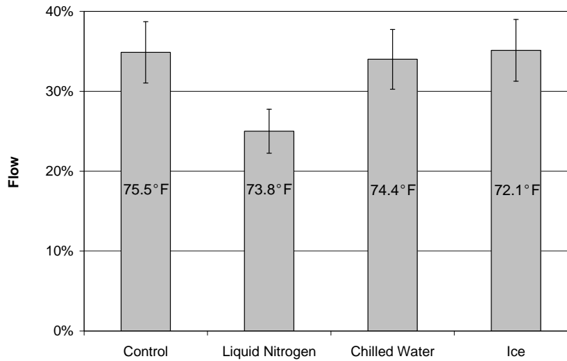
Figure 3.2 Flow of cement mortar containing Pozzolith 200N
