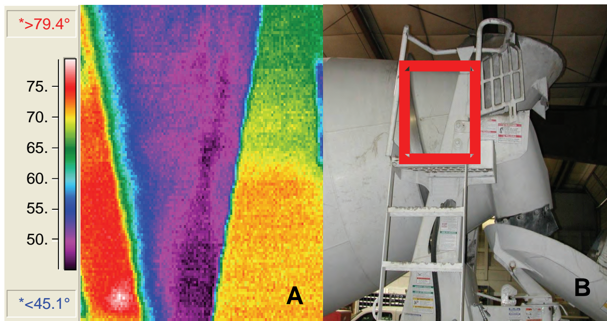
Figure 8.3 Thermal image (A) of a steel mixing drum during liquid nitrogen dosing. In B the area in red indicates the region of a mixing drum that the image is capturing.
