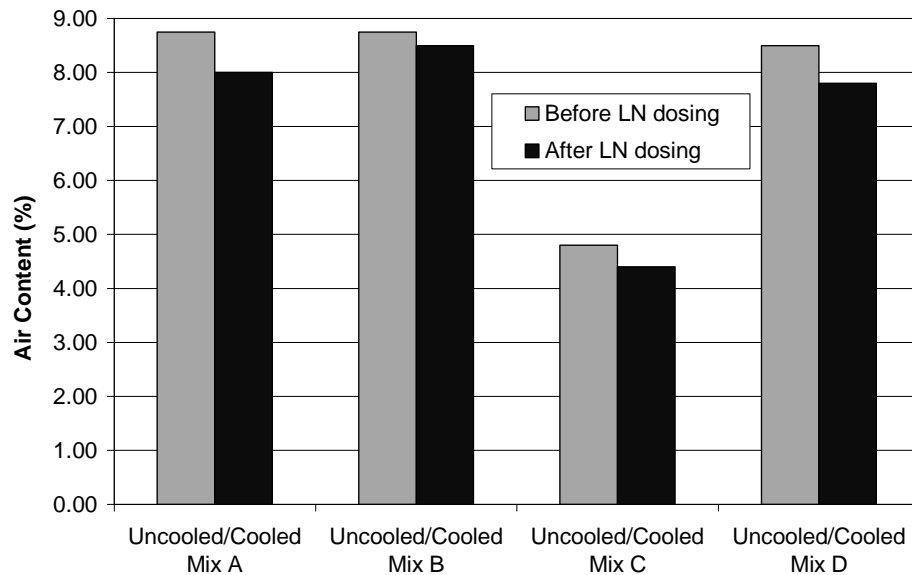
Figure 7.2 Fresh air contents for field-mixed concrete
