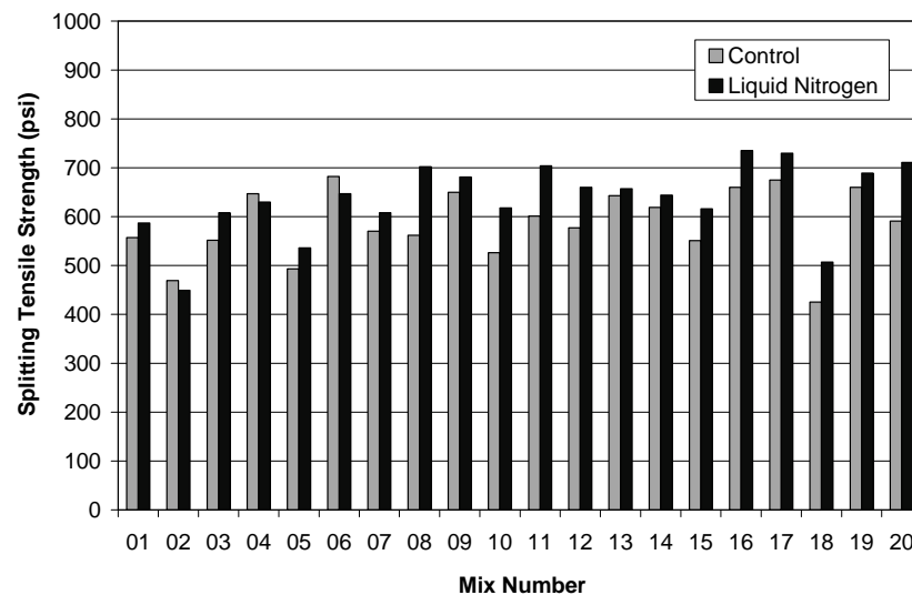
Figure 4.5 28-day splitting tensile strengths for laboratory-mixed concrete
