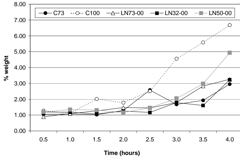
Figure 5.7 Calcium hydroxide analyses by x-ray diffraction for five mixtures
