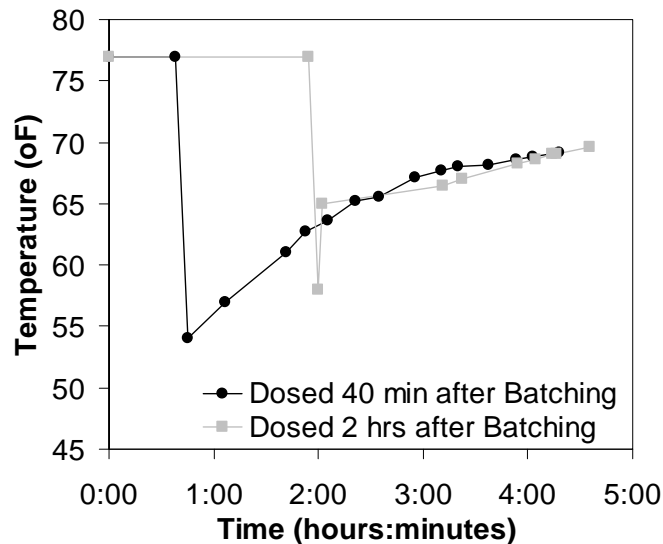
Figure 6.5 Temperature results of delayed dosing of field concrete
