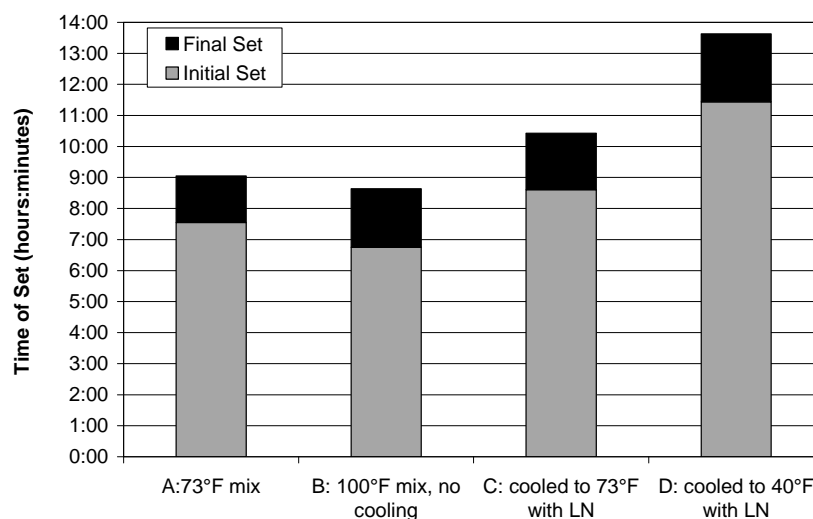
Figure 3.9 Effect of temperature on the setting time of concrete
