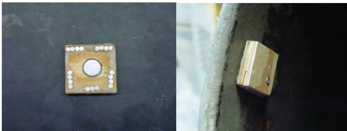
Figure 8.4 a. iButton temperature sensor in protective casing; b. iButton sensor attached to the side of a laboratory mixing drum
