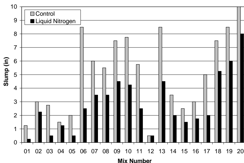
Figure 3.5 Slump results for room temperature and liquid nitrogen cooled concrete
