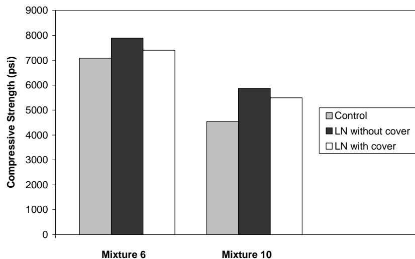
Figure 4.3 28-day compressive strengths of room temperature, covered, and uncovered concrete
