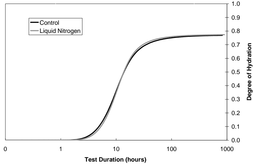
Figure 5.2 Degree of hydration curves from semi-adiabatic calorimetry for Mixture 8 (air entrainer + water reducer)
