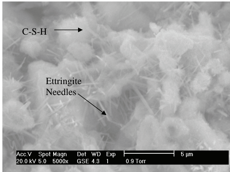
Figure 5.13 ESEM image of fractured cement paste surface from mixture LN73-00 after 24 hours of hydration
