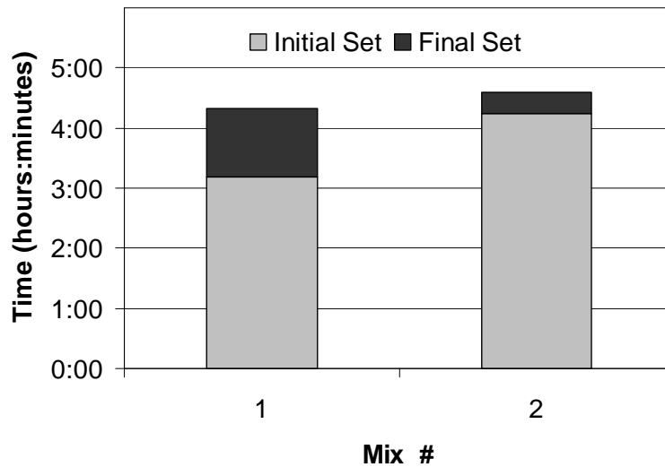
Figure 6.4 Setting time results of delayed dosing of field concrete with one batch dosed after 40 minutes (“1”) and another dosed at 2 hours (“2”)
