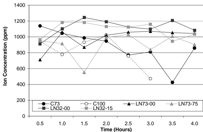
Figure 5.9 Calcium concentrations for six different cement paste mixtures
