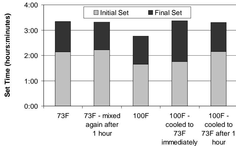
Figure 6.2 Setting time of cement pastes with initial temperatures of 73°F and 100°F, cooled to 73°F immediately or after a 1 hour delay
