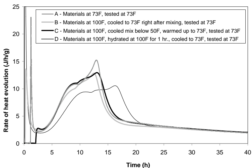
Figure 5.4 Heat evolution curves for isothermal calorimetry Mixture 4, A-D (C ash)
