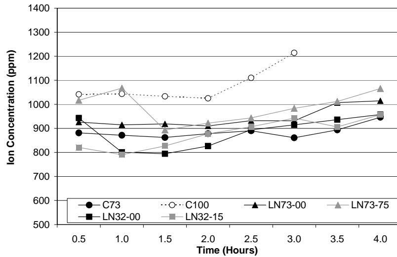
Figure 5.10 Sulfur concentrations for six different cement paste mixtures
