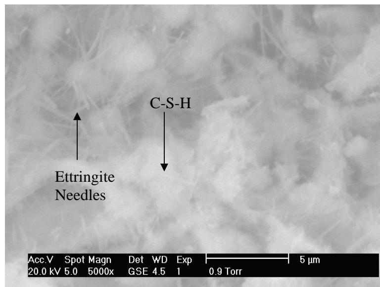
Figure 5.16 ESEM image of fractured cement paste surface from mixture LN32-00 after 24 hours of hydration
