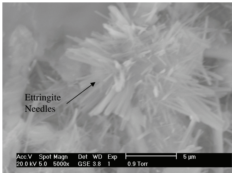
Figure 5.14 ESEM image of fractured cement paste surface from mixture LN73-105 after 24 hours of hydration
