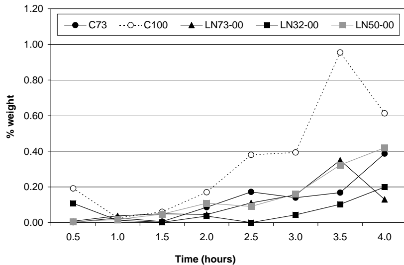
Figure 5.8 Monosulfoaluminate analysis by x-ray diffraction for five mixtures
